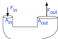
Figure 1: Hydraulic lift.
